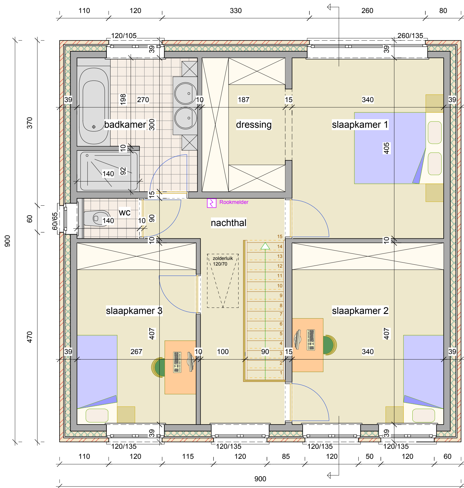
Plan VERDIEPING
